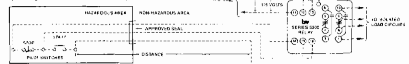
Series 53 relay with intrinsically safe holding circuit operating from the contacts of two pilot switches.
